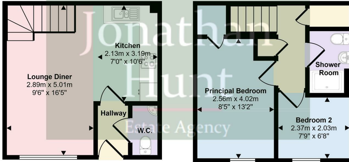
Ground Floor Approx 25 sq m / 274 sq ft
